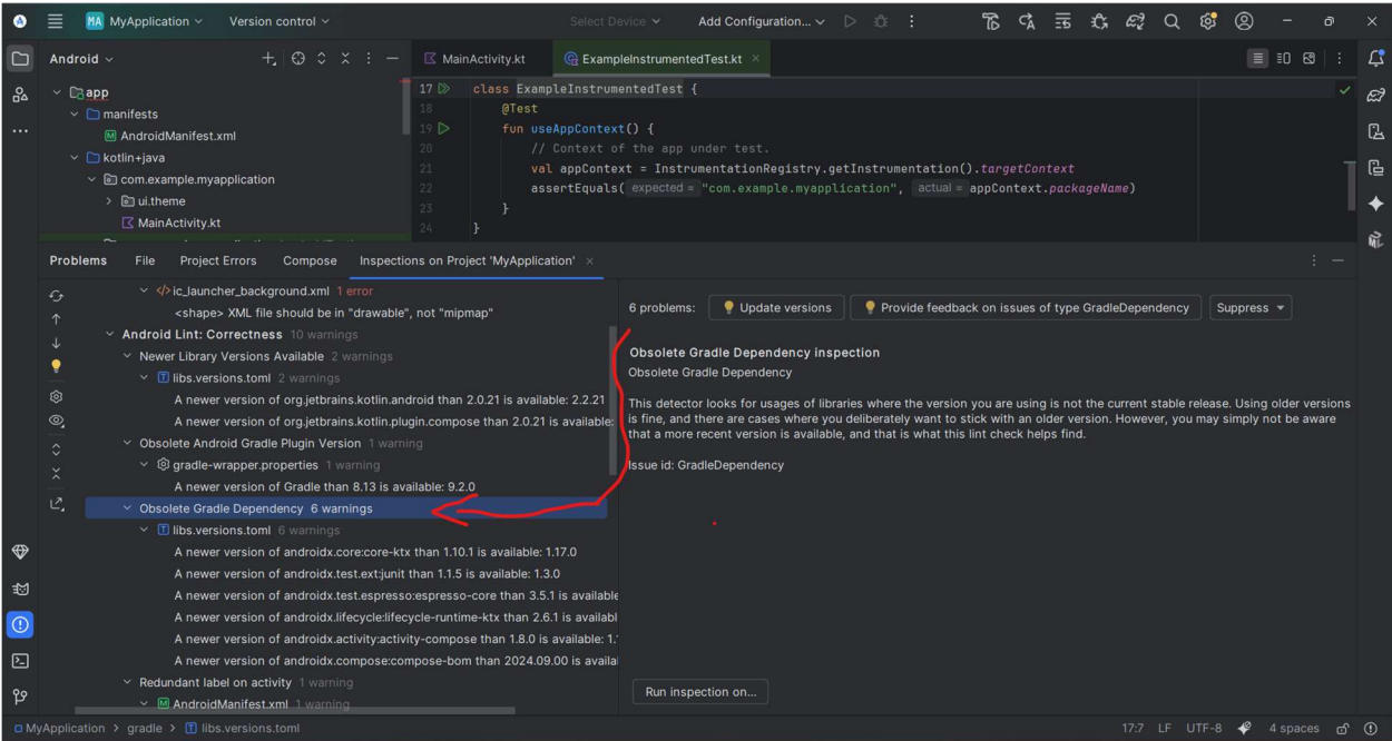
Figure 2: (Obsolete Gradle Dependency)
