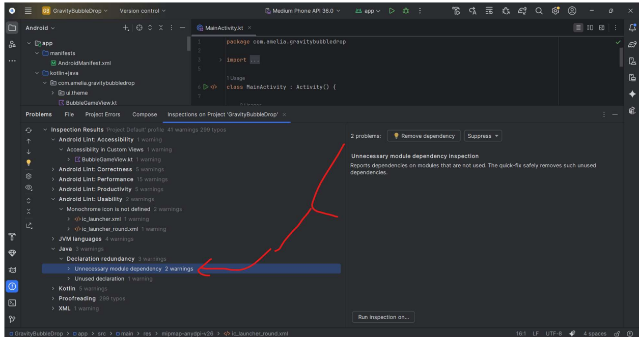
Figure 4: Declaration Redundancy – Unnecessary Module Dependency
