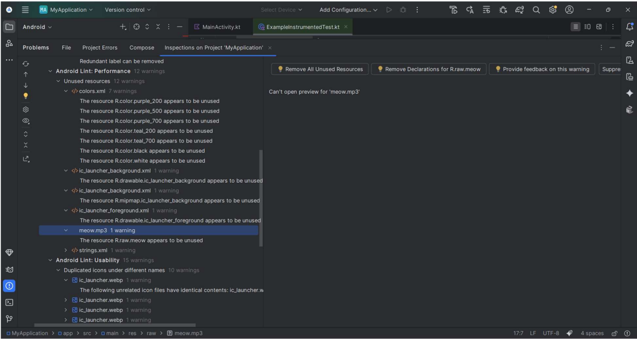
Figure 5: Performance – Unused Resources
