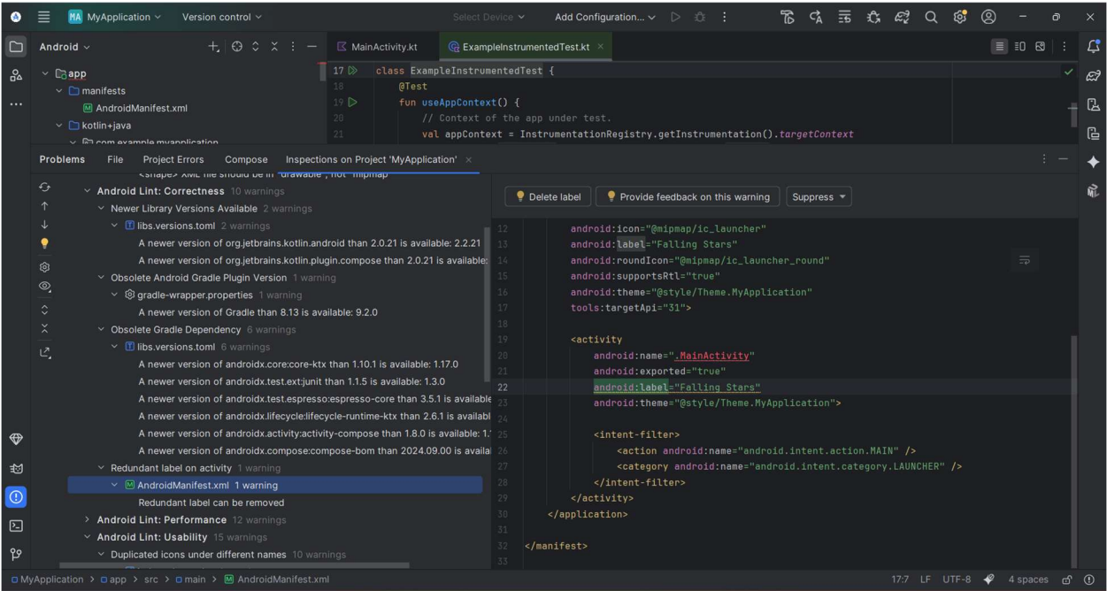
Figure 3 (Redundant label on activity)
