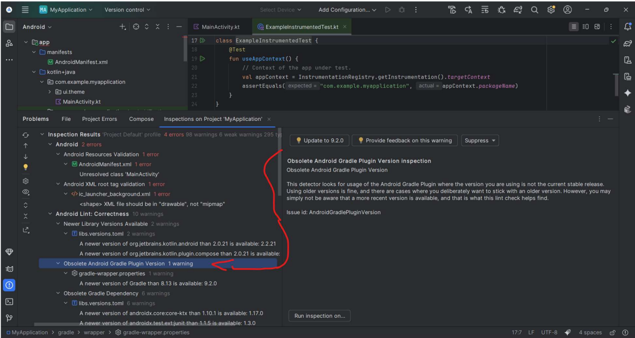
Figure 1: (Obsolete Android Gradle Plugin Version)
