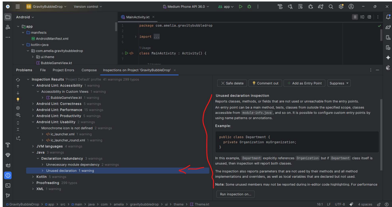
Figure 5: Declaration Redundancy – Unused Declaration
